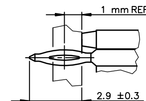
DETAIL-1: PRESS-FIT TAIL
