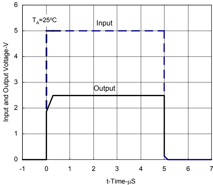
Pulse Response
