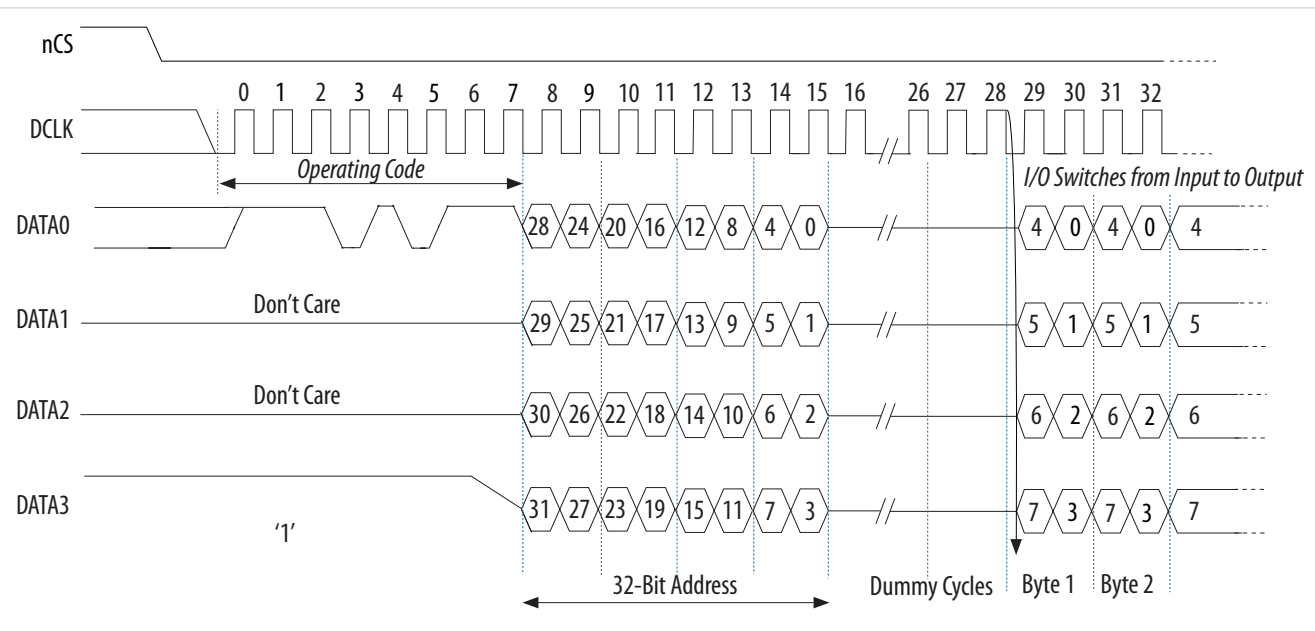
Figure 13: Extended Quad Input Fast Read Operation
