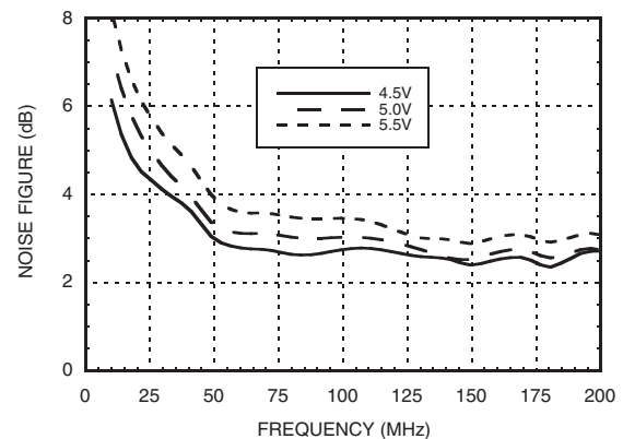
Noise Figure vs. V dd for Low Frequencies [1][2]
