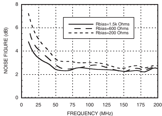
Noise Figure vs. Rbias for Low Frequencies [1][2]
