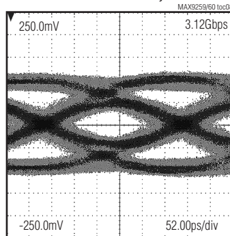
SERIAL LINK SWITCHING PATTERN WITH 14dB PREEQUALIZATION (PARALLEL BIT RATE = 104MHz, 10m STP CABLE)
