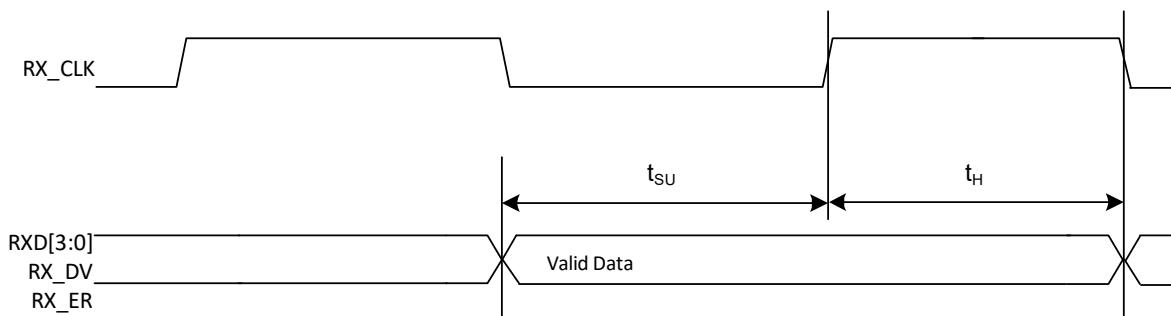
Figure 26 • MII Receive Timing
