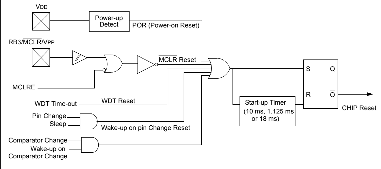
FIGURE 8-8: TIME-OUT SEQUENCE ON POWER-UP ( \overline{\text{MCLR}} PULLED LOW)
