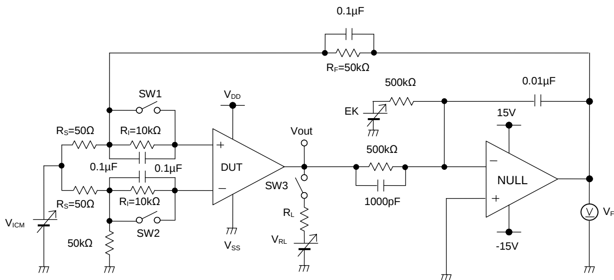
Figure 67. Test Circuit1
