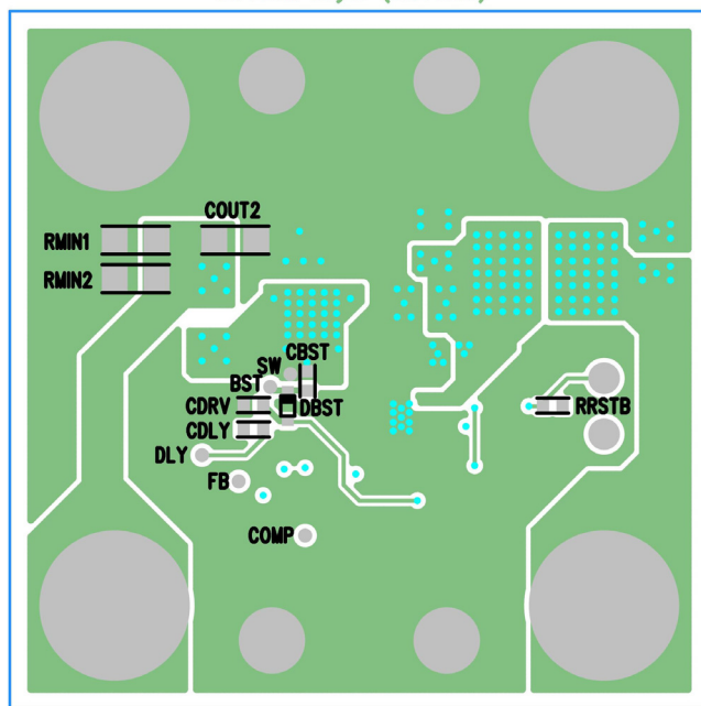
Figure 15. Bottom View
