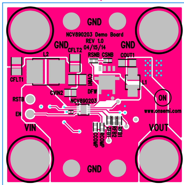
Figure 14. Top View
