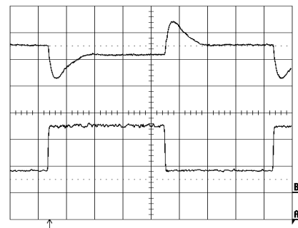
Output voltage response to load current step-change (8.25-24.75-8.25 A) at: T_{P1} = +25^{\circ}\text{C} , V_1 = 53\text{ V} , C_o = 3.3\text{ mF} .
