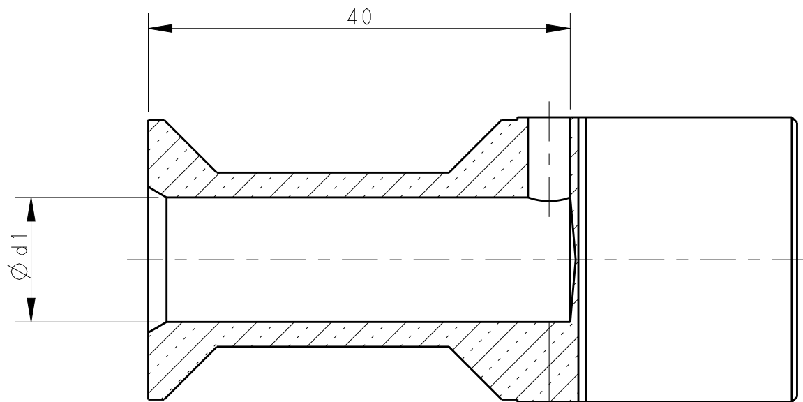
SECTION B-B
