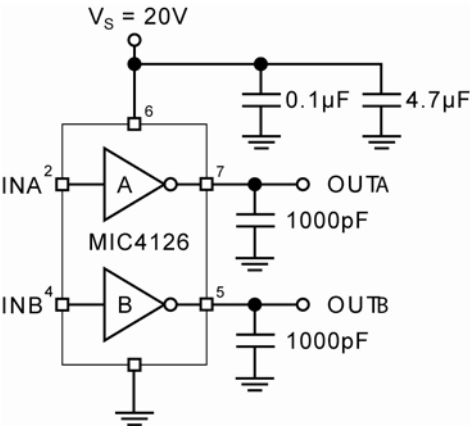
Figure 1a. Inverting Configuration
