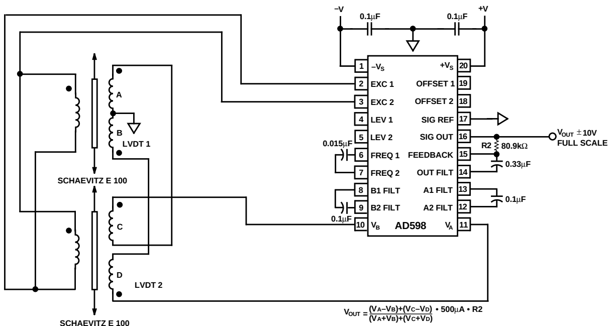
Figure 25. Differential Gaging
