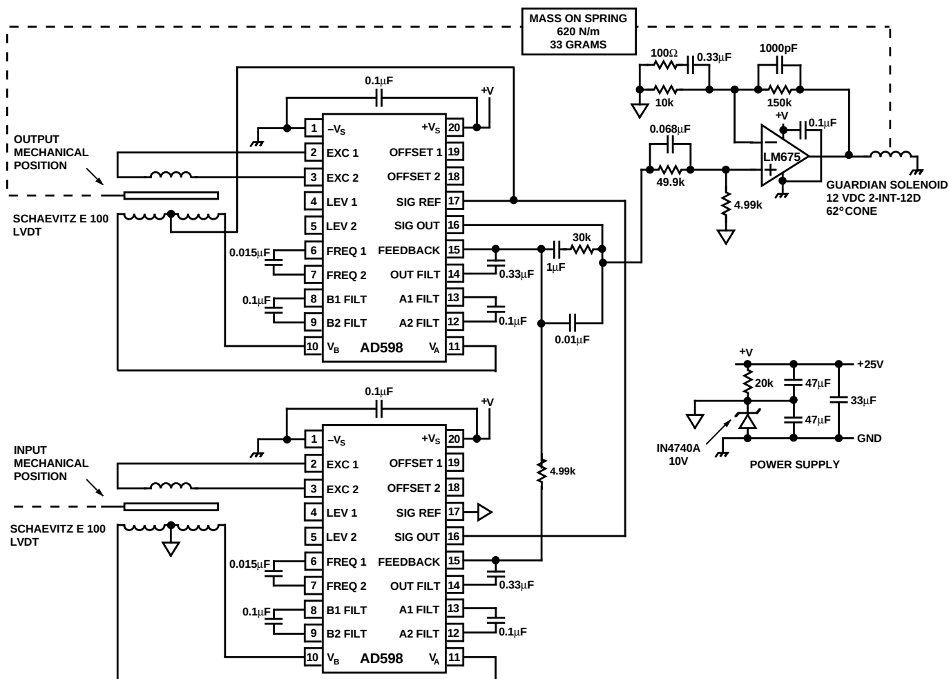
Figure 24. Mechanical Follower Servo-Loop
