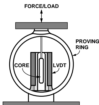
Figure 20. Proving Ring-Weigh Scale Cross Section
