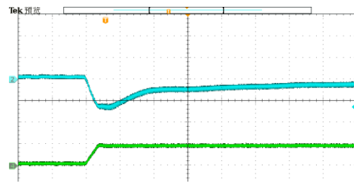
Figure 14. Load Transient V1, 8.45 to 92.95 A, 1A/uS (200 \mu s/div) CH2: V1 (200mV/div) CH4: I1 (100A/div)
