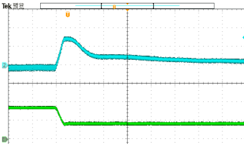
Figure 15. Load Transient V1, 169 to 84.5 A, 1A/uS (200 \mu s/div) CH2: V1 (200mV/div) CH4: I1 (100A/div)
