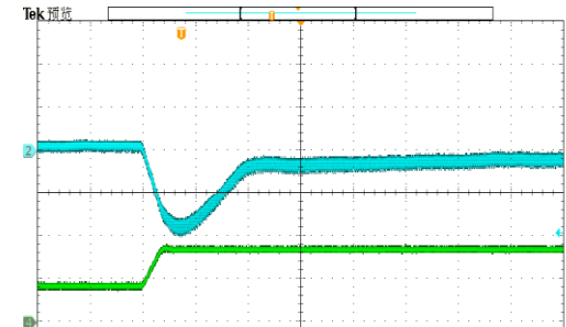
Figure 16. Load Transient V1, 84.5 to 169 A, 1A/uS (200 \mu s/div) CH2: V1 (200mV/div) CH4: I1 (100A/div)
