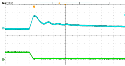
Figure 13. Load Transient V1, 92.95 to 8.45 A, 1A/uS (200 \mu s/div) CH2: V1 (200mV/div) CH4: I1 (100A/div)
