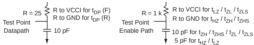
Figure 2-15 • AC Loading
