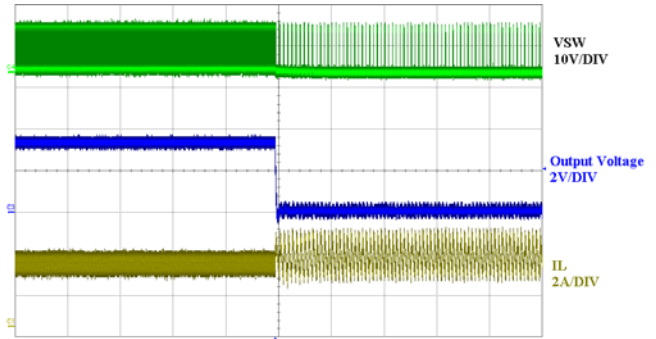
Figure 6. Short-Circuit Protection 200 μs/DIV
