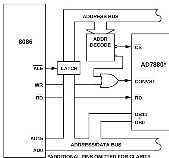
Figure 19. AD7880–8086 Interface
