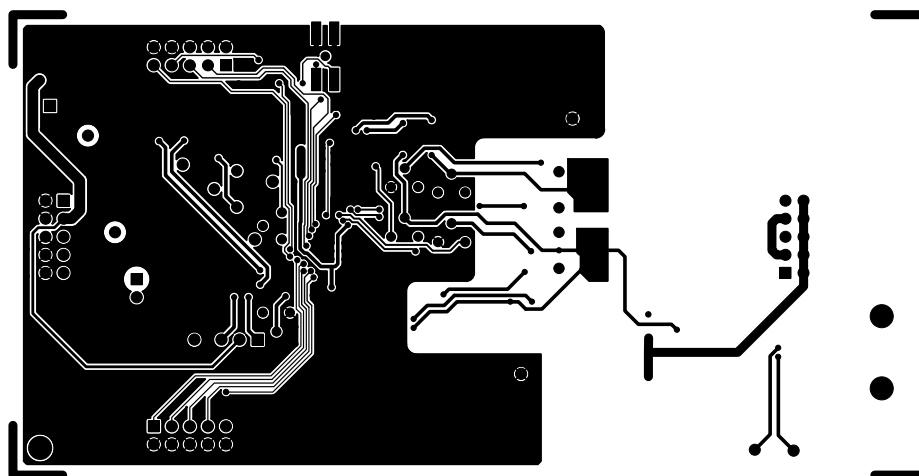
Figure 12. Si321xFM-DCX-EVB with Discretes Secondary Side
