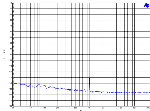
Figure 6. Crosstalk
