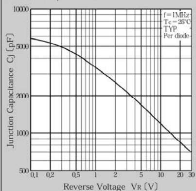
Junction Capacitance
