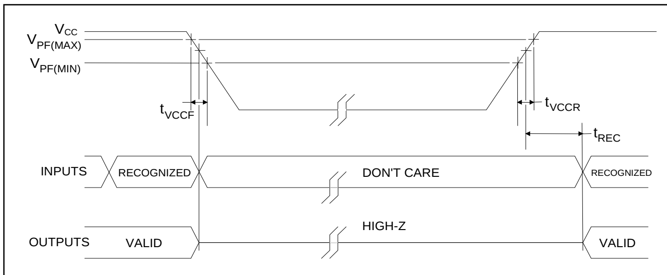
Figure 1. Power-Up/Down Timing
