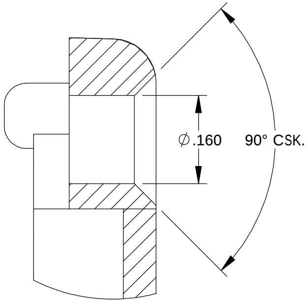
DETAIL D SCALE 6 : 1
