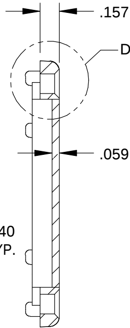
SECTION C-C
