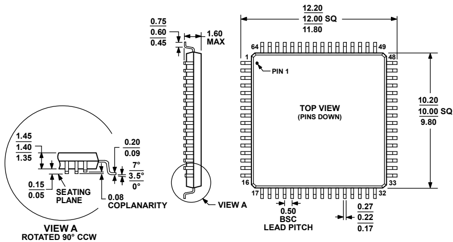
COMPLIANT TO JEDEC STANDARDS MS-026-BCD Figure 62. 64-Lead Low Profile Quad Flat Package [LQFP] (ST-64-2) Dimensions shown in millimeters
