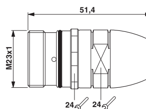
Dimensional drawing
