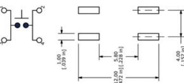
SCHEMATIC
