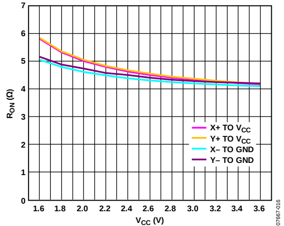
Figure 16. Switch On Resistance vs. V_{CC} (X+, Y+: Pin to V_{CC} ; X-, Y-: Pin to GND)
