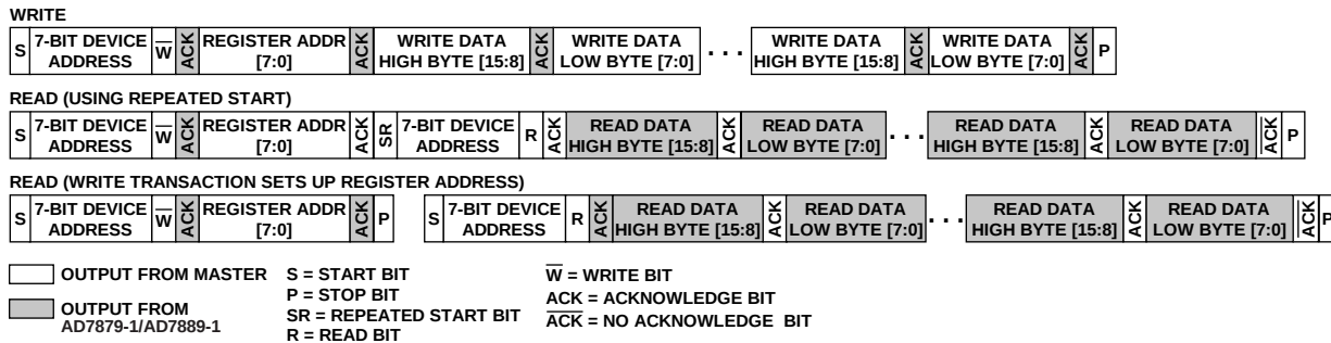
Figure 45. Example of Sequential I 2 C Write and Readback Operation
