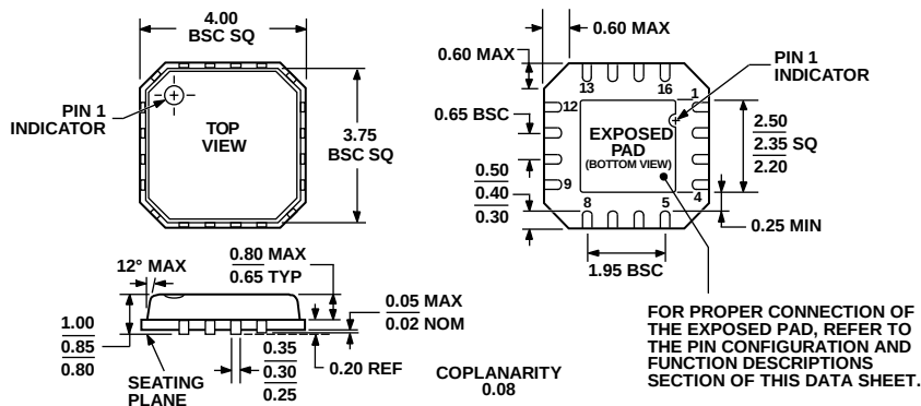
Figure 49. 16-Lead Lead Frame Chip Scale Package [LFCSP_VQ] 4 mm x 4 mm, Very Thin Quad (CP-16-10) Dimensions shown in millimeters
