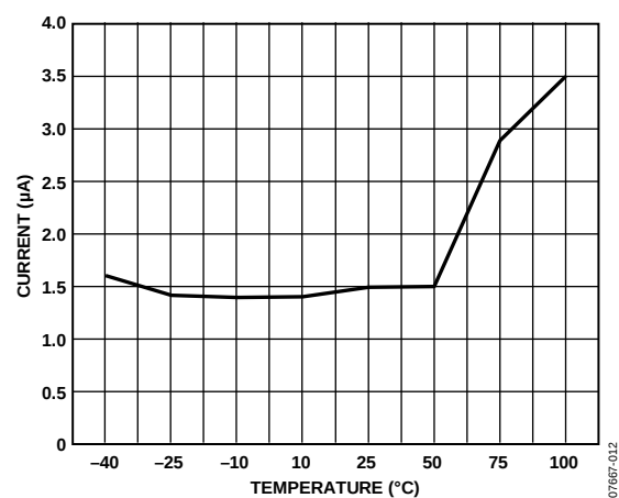
Figure 11. Full Power-Down I_{DD} vs. Temperature
