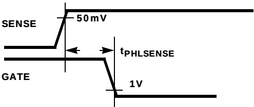
FIGURE 2. SENSE TO GATE TIMING
