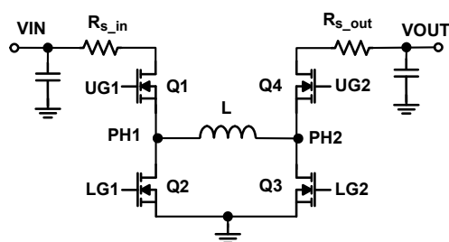
Figure 1. Buck-Boost Power Train Topology
