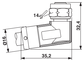
Dimensional drawing
