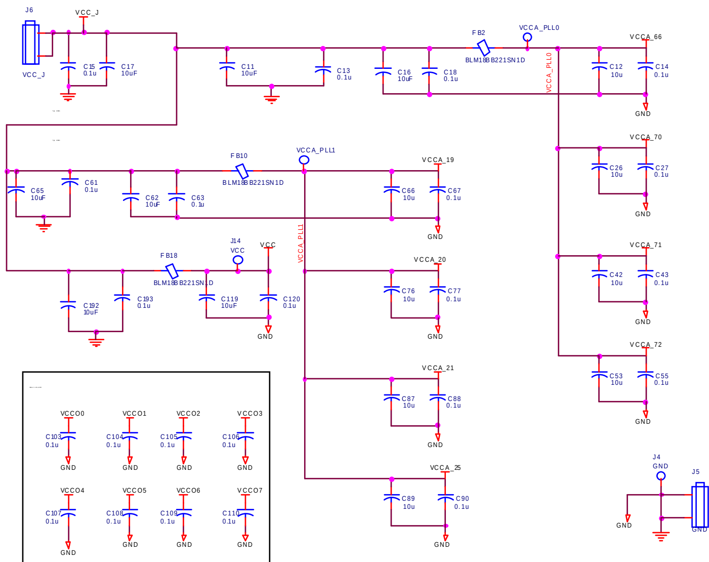
Figure 9. VCC Filtering
