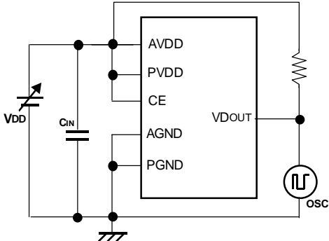
VD Detect and Release Voltage Test Circuit
