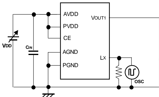
VD Detect and Release Voltage Test Circuit
