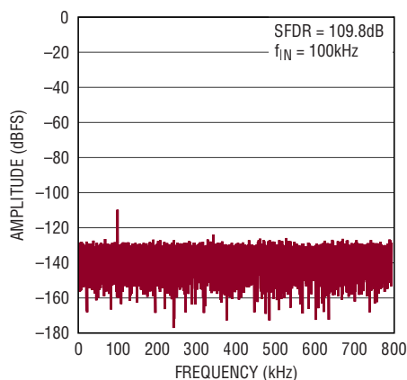
Crosstalk FFT (AC Crosstalk- Channel Adjacent to MUXOUT)
