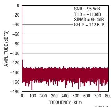
Figure 10b. 32k Point FFT f_{\text{SAMPL}} = 1.6\text{Mpsps} , f_{\text{IN}} = 1\text{kHz} for Circuit Shown in Figure 10a
