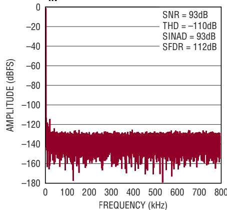
32k Point FFT f_{\text{SAMPL}} = 1.6\text{Msps} , f_{\text{IN}} = 1\text{kHz}
