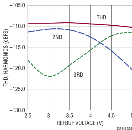
THD, Harmonics vs \text{REFBUF} , f_{\text{IN}} = 1\text{kHz}
