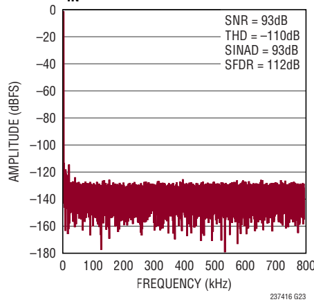
32k Point FFT f_{\text{SAMPL}} = 1.6\text{MSPS} , f_{\text{IN}} = 1\text{kHz}
