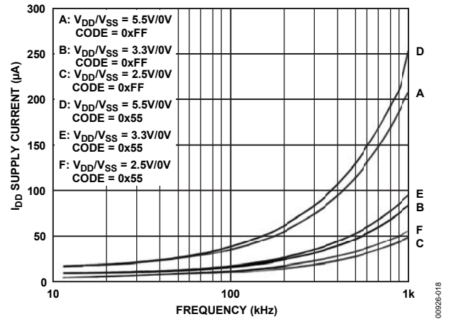
Figure 18. Supply Current vs. Frequency
