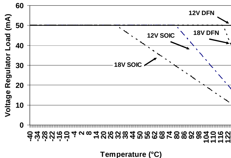
FIGURE 2-2: MCP2021-330 Safe Operating Range.
