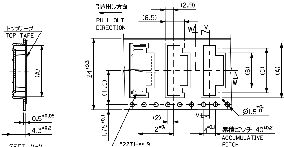
SECT. V-V
