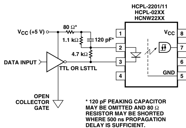
Figure 16. Series LED drive with open collector gate ( 4.7\ \text{k} resistor shunts I_{OH} from the LED).
