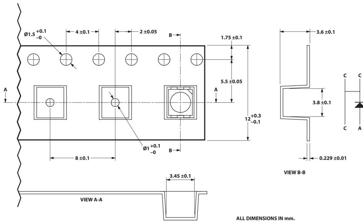
Figure 14: Tape Dimensions
