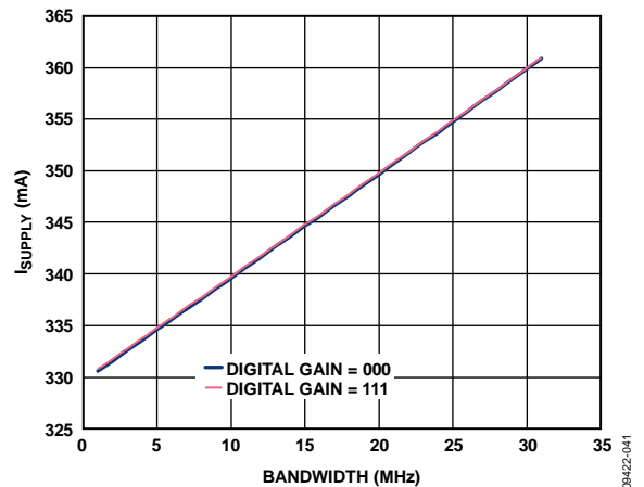
Figure 40. Current Consumption at Minimum and Maximum Digital Gain vs. Bandwidth (Bandwidth Setting = 31 MHz, Gain = 30 dB)
