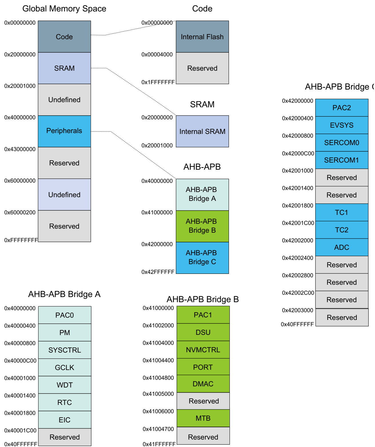
Figure 8-1. Atmel SAM D09 Product Mapping
