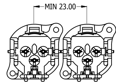
MIN MOUNTING PITCH SCALE 1:1
