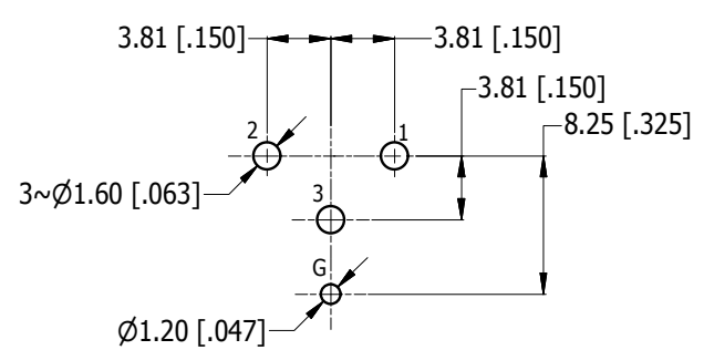
PCB-LAYOUT COMPONENT SIDE TOLERANCE: ± 0.05mm [.002"]
