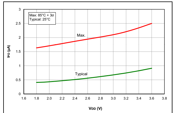
FIGURE 27-23: I_{PD} , Watchdog Timer (WDT), PIC16LF1703/7 only.
