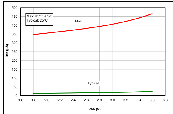
FIGURE 27-35: I_{PD} , ADC Non-Converting, PIC16LF1703/7 only
