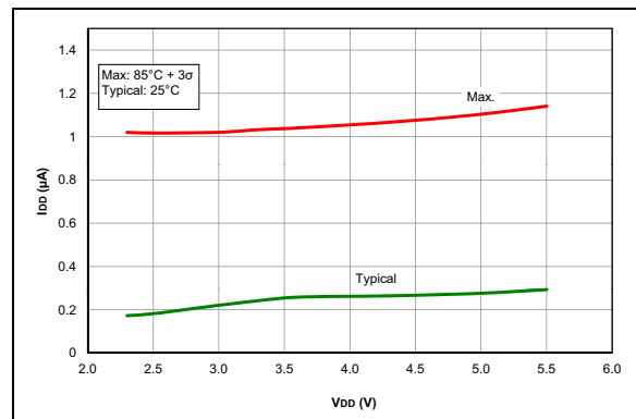
FIGURE 27-36: I_{PD} , ADC Non-Converting, PIC16F1703/7 only
