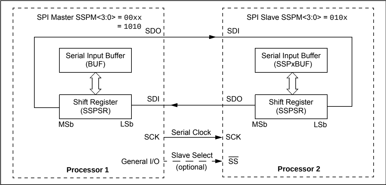
FIGURE 23-5: SPI MASTER/S�AVE CONNECTION
