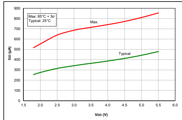
FIGURE 27-34: I_{PD} , Op Amp, High GBWP Mode ( OPAxSP = 1 ), PIC16F1703/7 Only.
