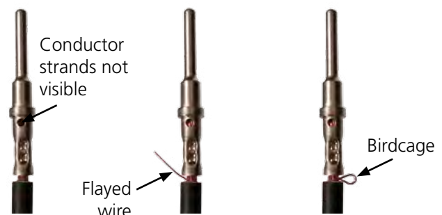
Unacceptable Crimps
