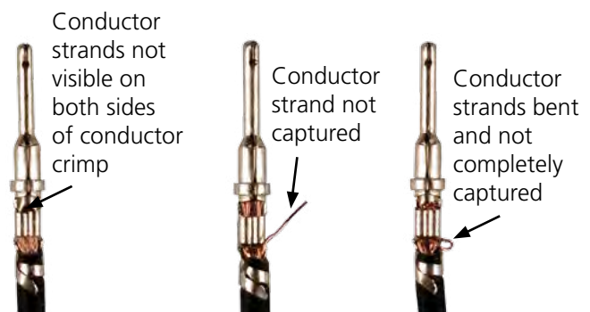
Unacceptable Crimps
