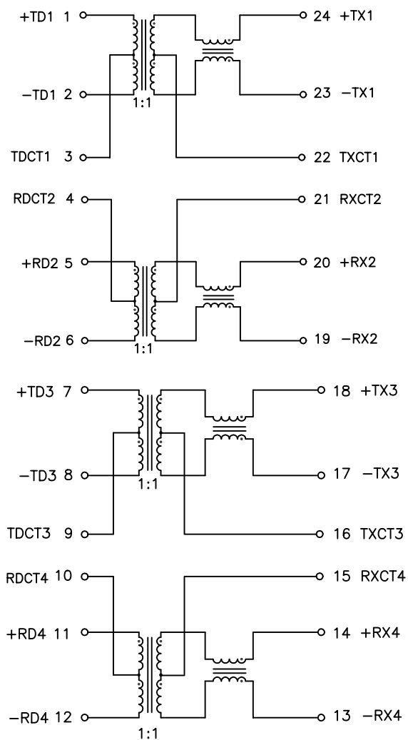
SCHEMATIC
