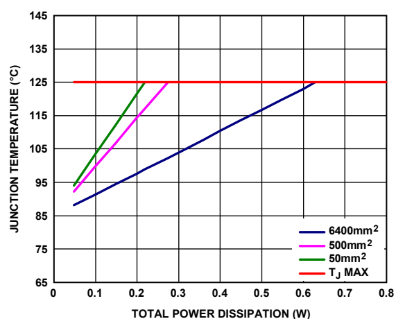
Figure 57. SOIC, T_A = 85^{\circ}\text{C}
