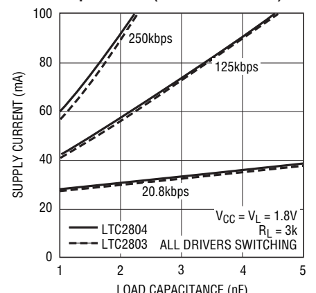
Supply Current vs Load Capacitance (Dual Transceiver)
